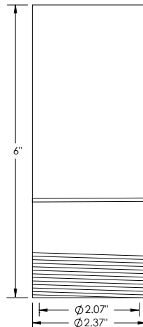
D-Lux: 32-D6-DCx (x = sign size)
