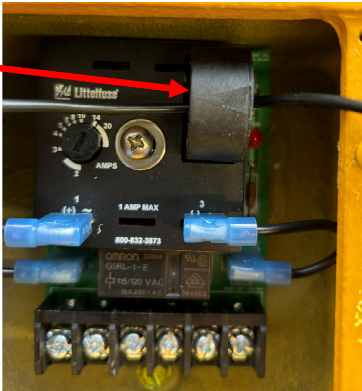
PHOTO 2 (L-864 Beacon Toroidal Transformer Wiring)
